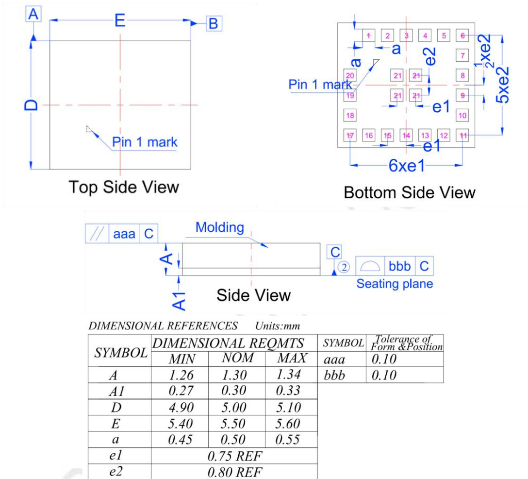
Figure 6.1: HJ-180IMH-11 dimension
